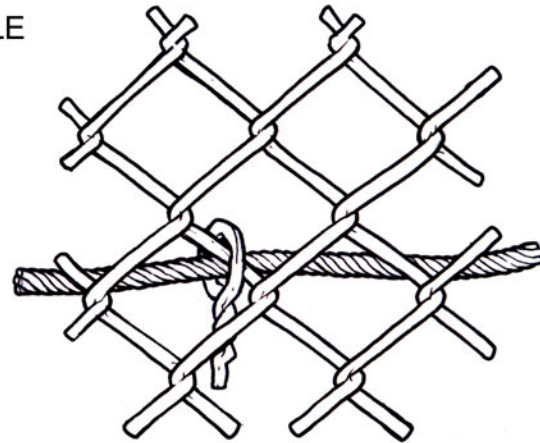
3/8" Cable
